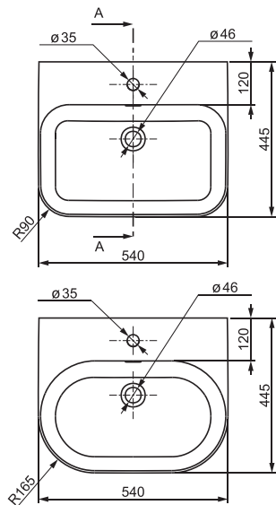
Ceramic Slim O 550 Wall N
