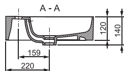
Ceramic Slim R 550 Wall N
