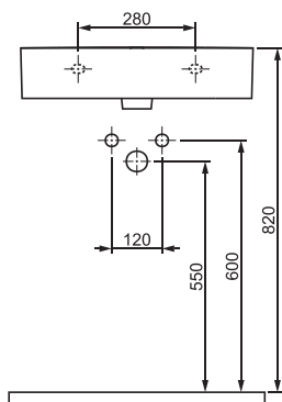
Ceramic Slim R 550 Wall N
